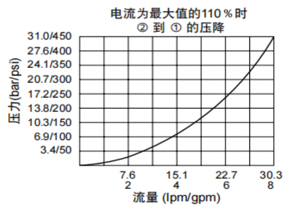
性能曲线图 Performance Characteristic Curve
