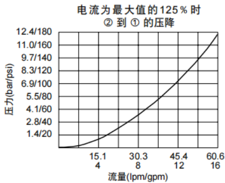
性能曲线图 Performance Characteristic Curve
