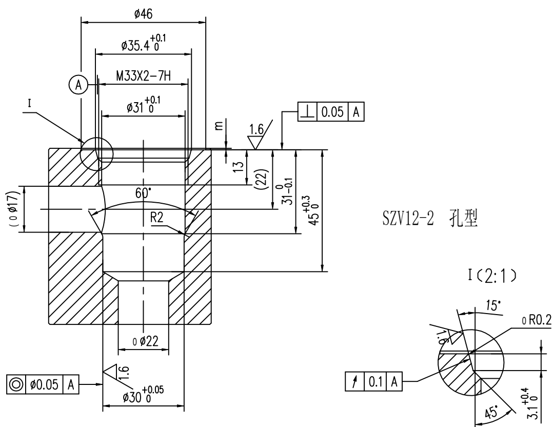
Hole Pattern Drawing
