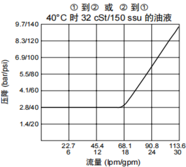
性能曲线图 Performance Characteristic Curve
