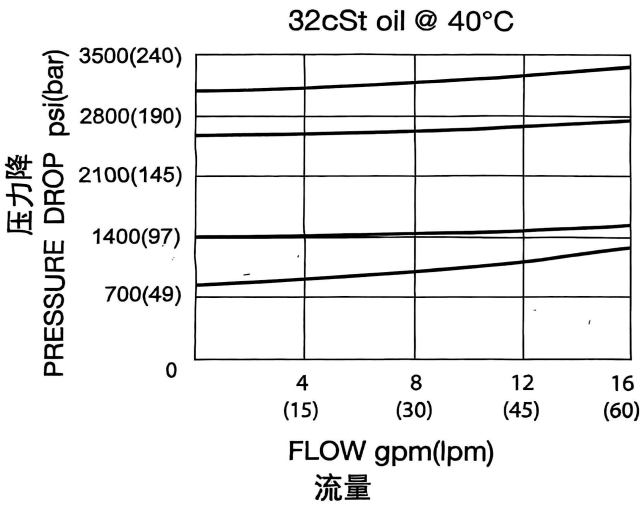
压力曲线图 Pressure Characteristic Curve
